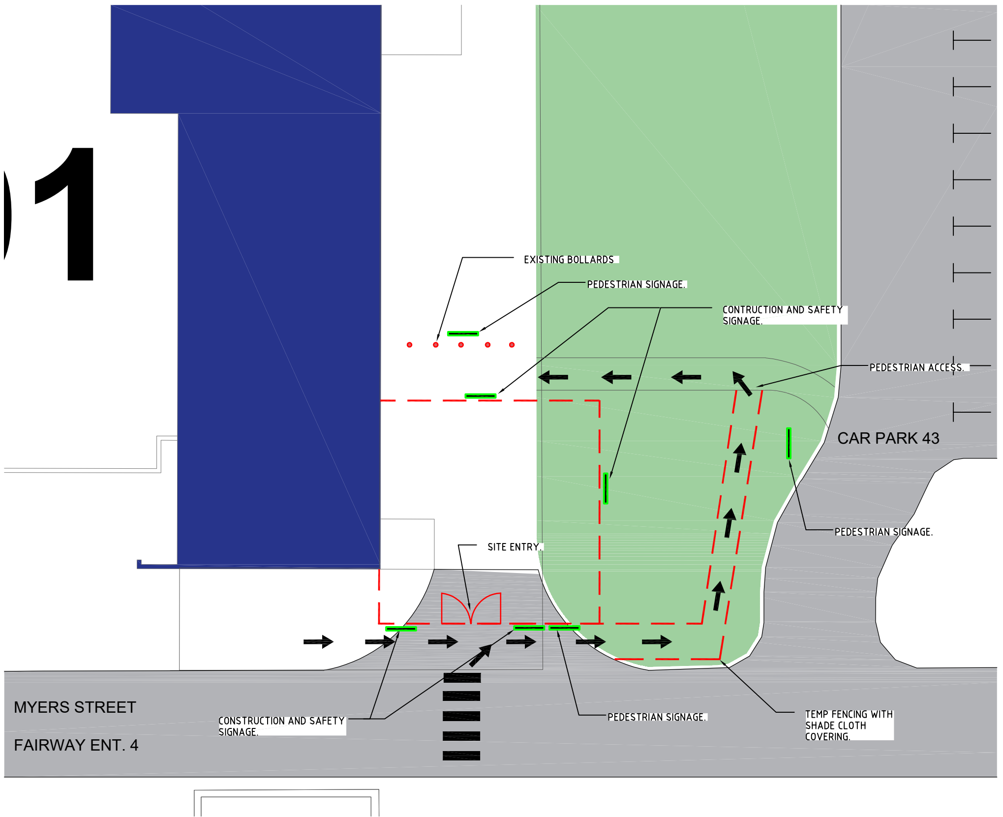
SITE & TRAFFIC PLAN
